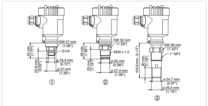
Dimensions VEGABAR 54
