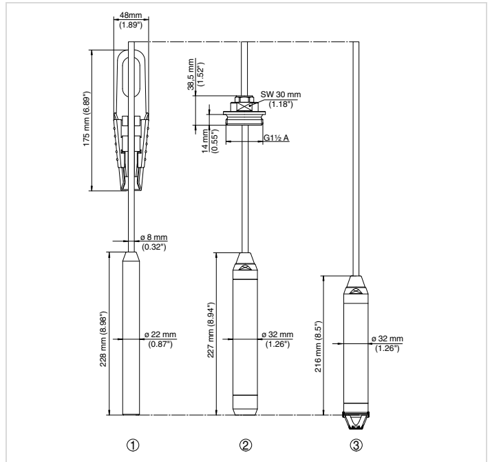
Dimensions VEGAWELL 52
