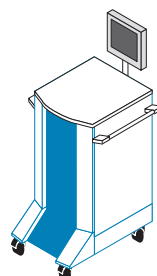
Mobile workstation/workshop trolley consisting of: ● Base/plinth with castors ● IW enclosure ● Worktop ● Handle system ● Operating housing
